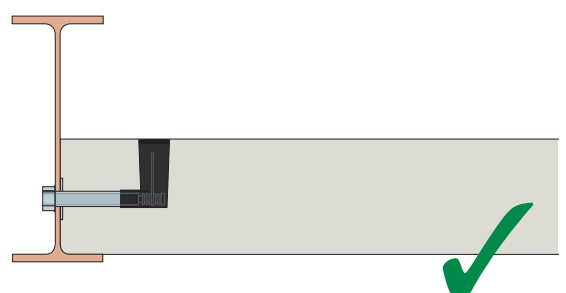
Ancon Lockable Dowel, in conjunction with Ancon Weldable Coupler. Contact Ancon with details of your project requirements.
