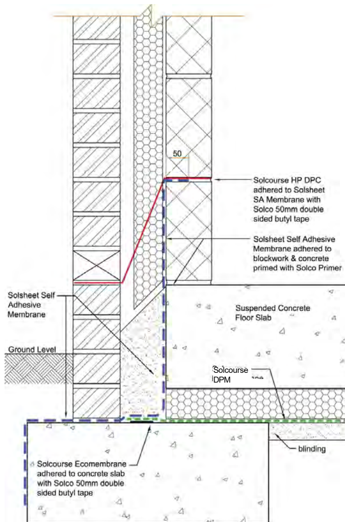
Typical Slab Edge Detail (Suspended) Standard Construction
