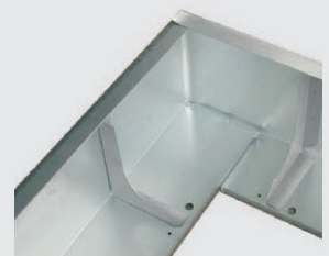
External Corner: Cut base & bend
